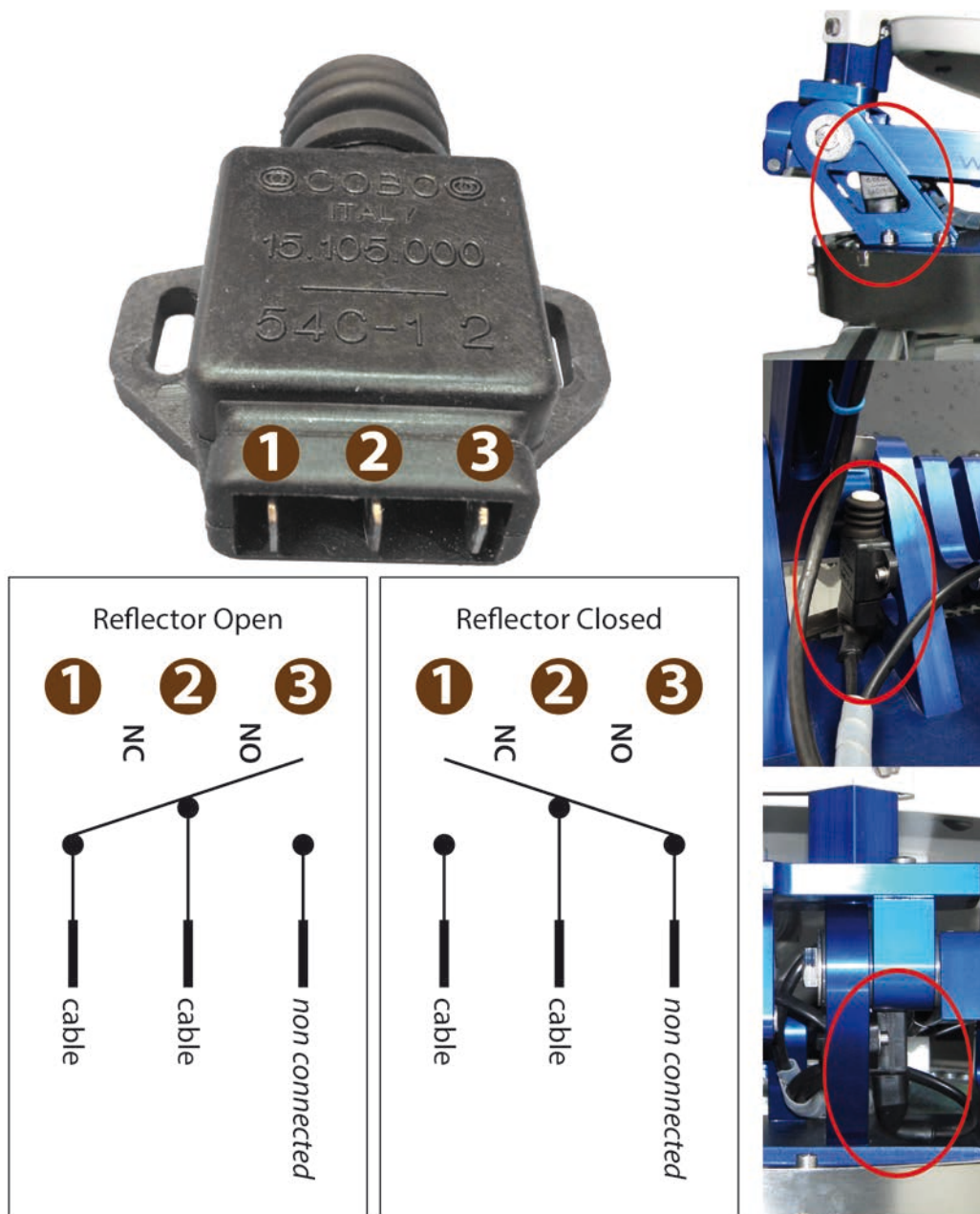
Pict.4-13 - Azimuth control switch
