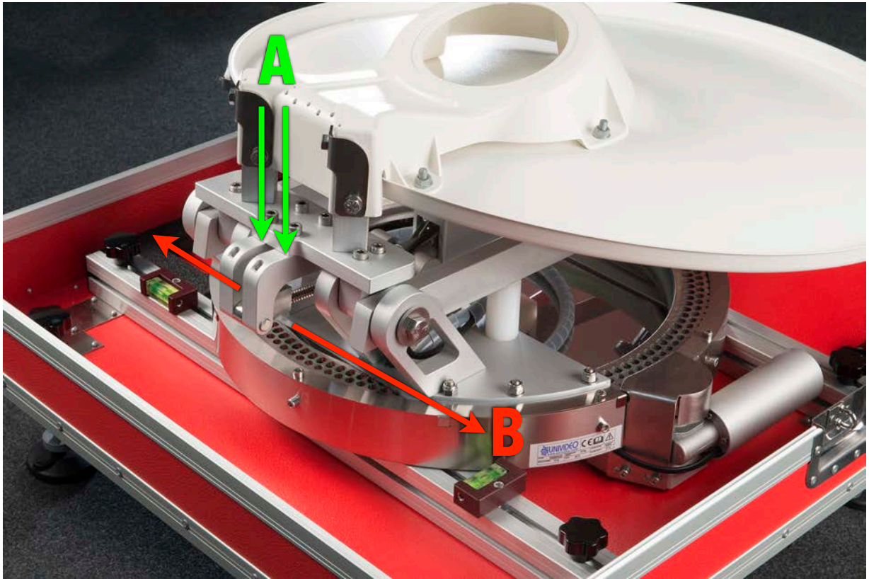
Pict.4-14 -Elevation motor uncouple
