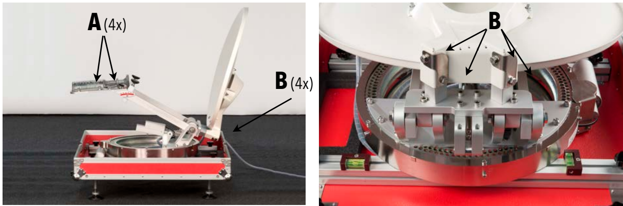
Pict.3-3 - Fixing SurfBeam ViaSat®2 kit: TRIA (A) and reflector (B)
