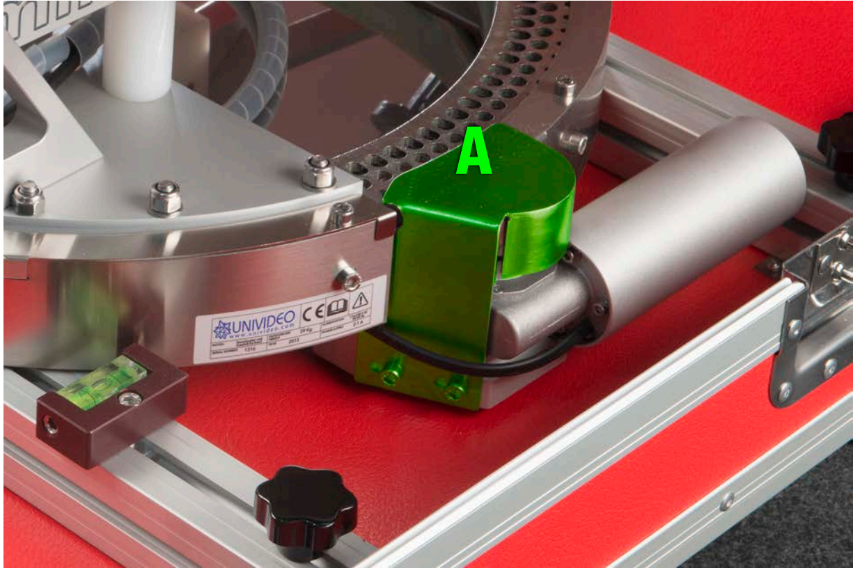
Pict.4-15 - Azimuth motor uncouple
